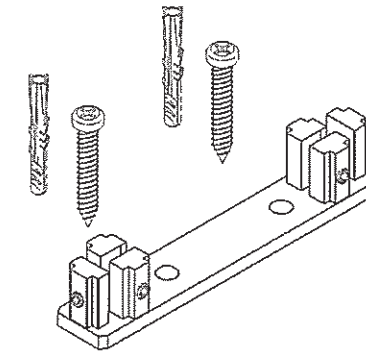
(A) Zinc Bracket (Inclusive of 2 Pan Head Tapping Screws & 2 Wall Plugs)
